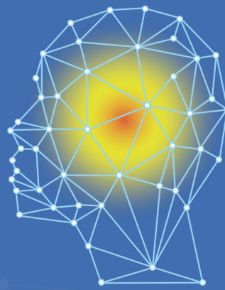
KNOWLEDGE
